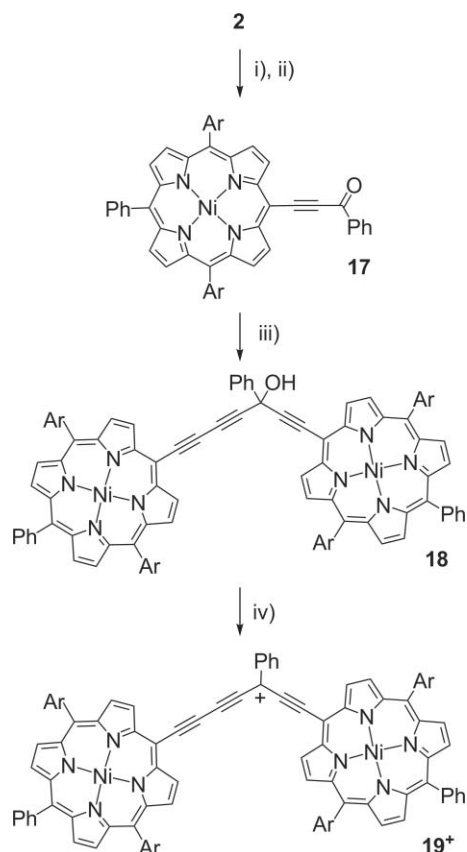
Scheme 4 Reagents and conditions: i) Bu 4 NF, CH 2 Cl 2 , 20 °C, quant. ii) PhC(O)N(OMe)Me, LiN(SiMe 3 ) 2 , THF, 20 °C, 83%; iii) 3 (after silyl deprotection), LiN(SiMe 3 ) 2 , THF, 20 °C, 30%; iv) CF 3 CO 2 H, CHCl 3 .
