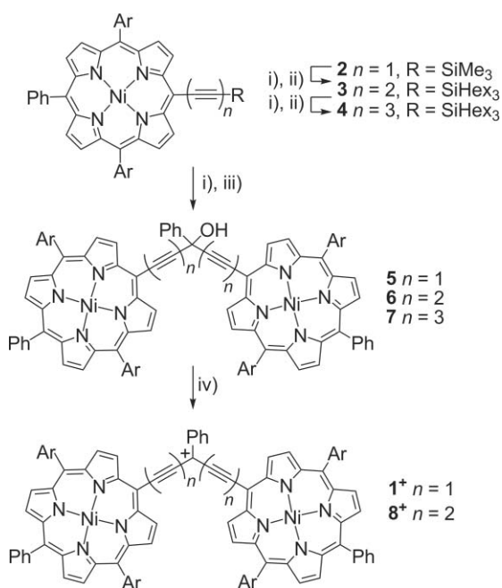
Scheme 1 Reagents and conditions: i) \text{Bu}_4\text{NF} , \text{CH}_2\text{Cl}_2 , 20\text{ }^\circ\text{C} , quant. ii) \text{HCCSiHex}_3 , \text{CuCl} , \text{TMEDA} , air, \text{CH}_2\text{Cl}_2 , \text{THF} , 20\text{ }^\circ\text{C} ( 3 : 91%; 4 : 95%); iii) \text{PhCO}_2\text{Me} , \text{LiN}(\text{SiMe}_3)_2 , \text{THF} , 20\text{ }^\circ\text{C} ( 5 : 53%; 6 : 31%; 7 : N/A); iv) \text{CF}_3\text{CO}_2\text{H} , \text{CHCl}_3 .
