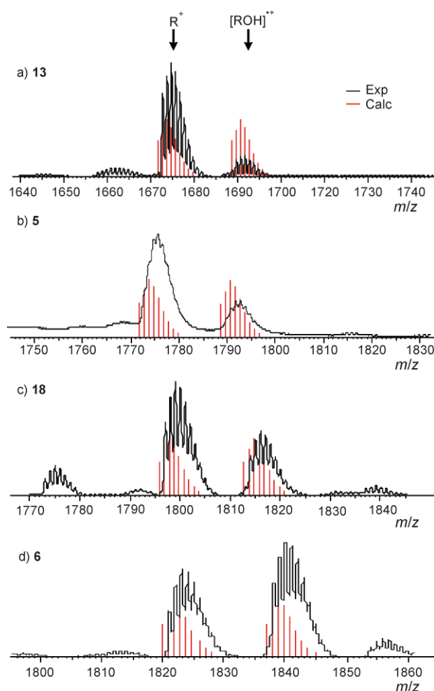
Fig. 5 MALDI-TOF spectra of porphyrin dimer alcohols ROH = 13 , 5 , 18 and 6 (a) to (d) respectively). The red lines show the calculated isotopic patterns for the alcohol [ROH] + and cation formed by protonation and dehydration R + in each case. Dithranol was used as the matrix.
