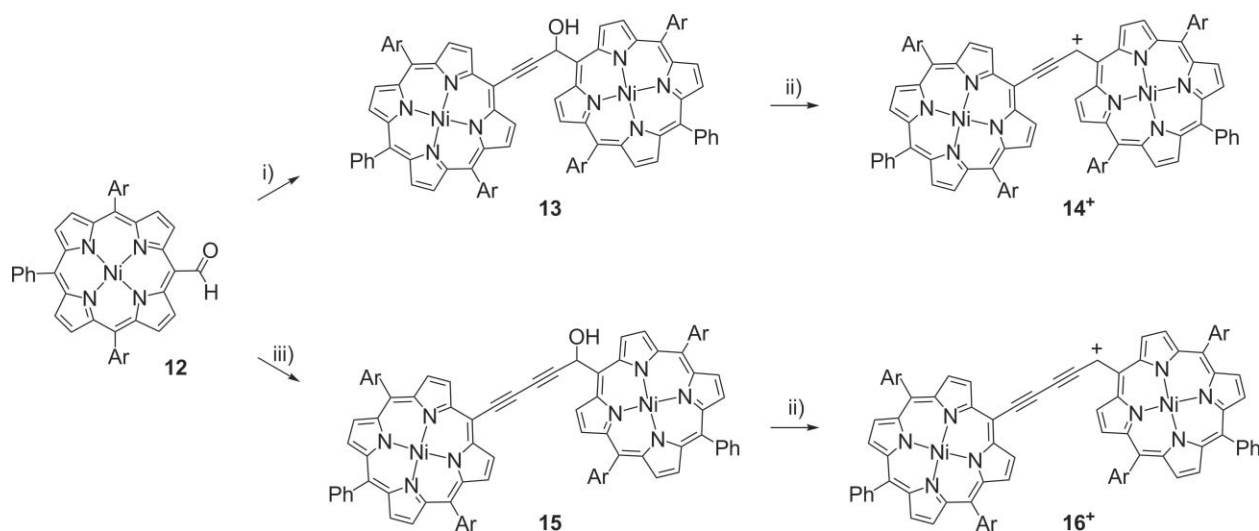
Scheme 3 Reagents and conditions: i) 2 (after silyl deprotection), \text{LiN}(\text{SiMe}_3)_2 , \text{THF} , 20\text{ }^\circ\text{C} , 30%; ii) \text{CF}_3\text{CO}_2\text{H} , \text{CHCl}_3 ; iii) 3 (after silyl deprotection), \text{LiN}(\text{SiMe}_3)_2 , \text{THF} , 20\text{ }^\circ\text{C} , 63%.
