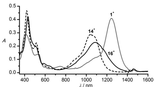
Fig. 3 Absorption spectrum of cations 14 + (C3, black dash), 16 + (unsymmetrical C5, black solid) and 1 + (symmetrical C5, grey solid) measured in CHCl 3 /2% TFA at 298 K.
