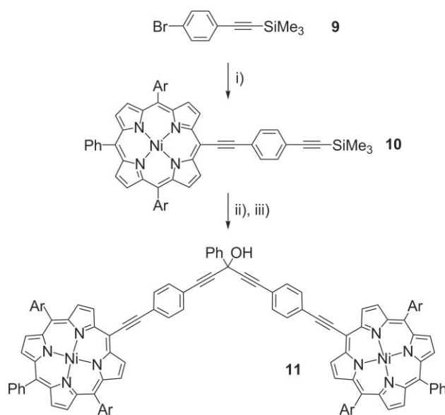
Scheme 2 Reagents and conditions; i) 2 , \text{Pd}_2(\text{dba})_3 , \text{PPh}_3 , \text{CuI} , \text{NEt}_3 , \text{PhMe} , 40\text{ }^\circ\text{C} , 48%; ii) \text{Bu}_4\text{NF} , \text{CH}_2\text{Cl}_2 , 20\text{ }^\circ\text{C} , quant. iii) \text{PhCO}_2\text{Me} , \text{LiN}(\text{SiMe}_3)_2 , \text{THF} , 20\text{ }^\circ\text{C} , 14%.
