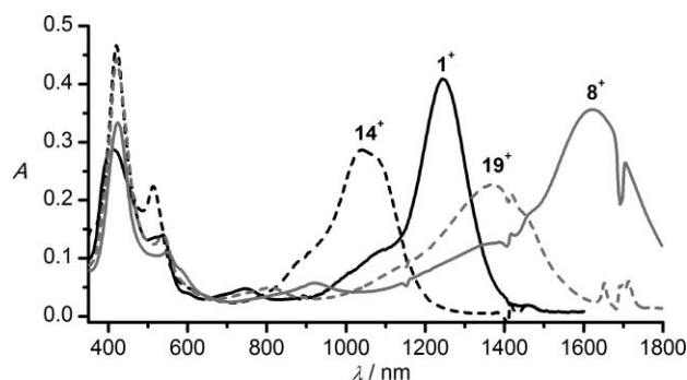
Fig. 2 Absorption spectra of cations 14 + (C3, black dash), 1 + (C5, black solid), 19 + (C7, grey dash) and 8 + (C9, grey solid) measured in CHCl 3 /2% TFA at 298 K. Spectra are normalised to the Soret maxima of the parent alcohols.
