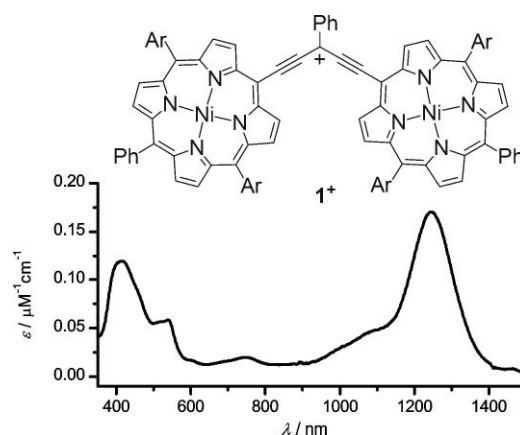
Fig. 1 Structure of cationic porphyrin dimer \mathbf{1}^+ and the UV/Vis/NIR spectrum measured in \text{CHCl}_3 /2% TFA at 298 K. Ar = 3,5-di- t -butyl phenyl.
