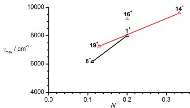
Fig. 4 Plot of \nu_{\max} against N^{-1} where N is the number of carbon atoms in the alkyne bridge. The lines join compounds of similar symmetry i.e. x = y (black), x = y + 1 (red) and x = y + 2 (green). \nu_{\max} is the frequency of the peak of the absorption band, measured in CHCl 3 /2% TFA.
